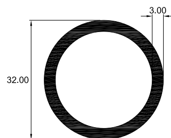
5609 TUBO CIRCULAR
