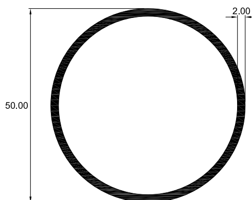
6705 TUBO CIRCULAR
