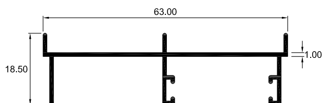
2009 JAMBA
