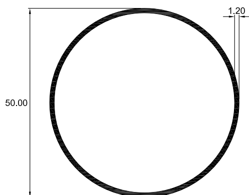
6704 TUBO CIRCULAR
