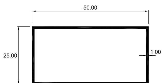
5222 TUBO RECTANGULAR
