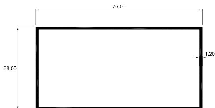
6426 TUBO RECTANGULAR
