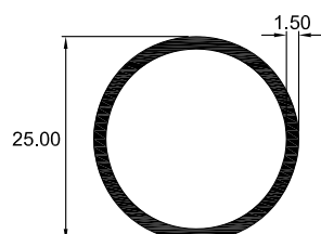
5568 TUBO CIRCULAR
