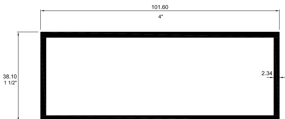
5142 TUBO RECTANGULAR
