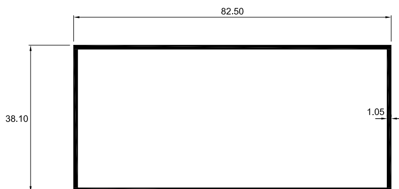
5231 TUBO RECTANGULAR
