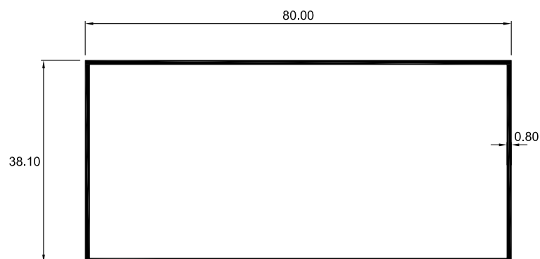
5232 TUBO RECTANGULAR
