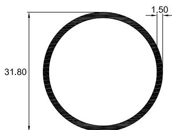
5611 TUBO CIRCULAR
