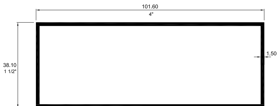
5242 TUBO RECTANGULAR
