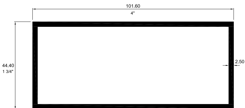
5243 TUBO RECTANGULAR
