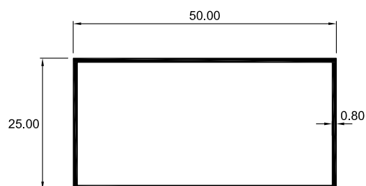
5221 TUBO RECTANGULAR
