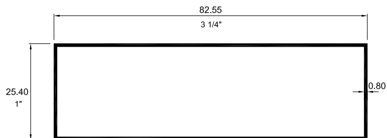
8656 TUBO RECTANGULAR
