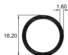
5535 TUBO CIRCULAR
