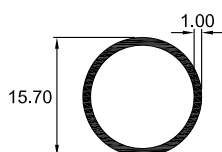
5524 TUBO CIRCULAR
