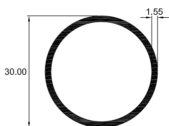
5610 TUBO CIRCULAR
