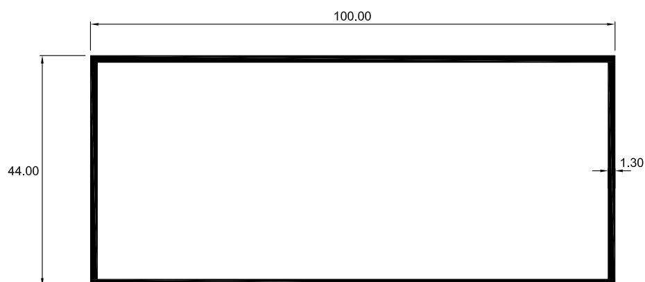
5241 TUBO RECTANGULAR
