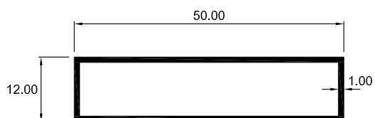
5219 TUBO RECTANGULAR
