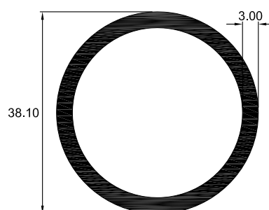
5662 TUBO CIRCULAR
